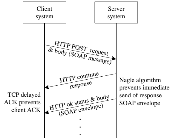
Fig. 4. Event trace of Microsoft SOAP communication.
