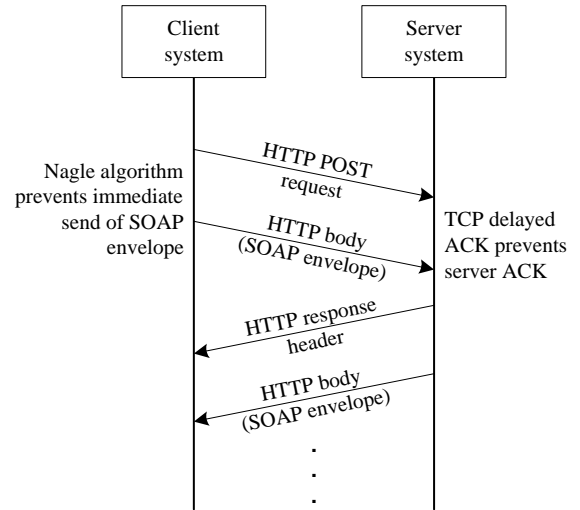
Fig. 3. Event trace of SOAP communication
